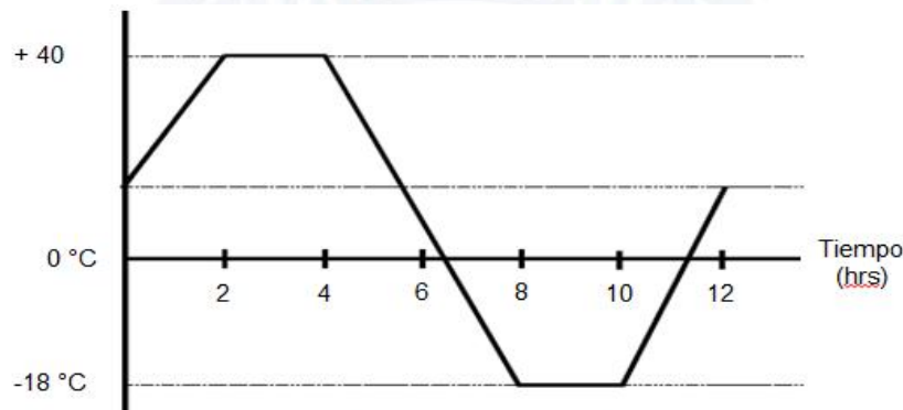
Fig. 6. IEC 61300-2-22, IEC 60068-2-14: Temperature Cycle Ageing
